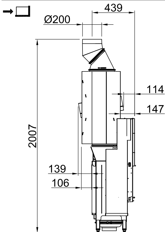
~1:20 Thermobox, schmal
