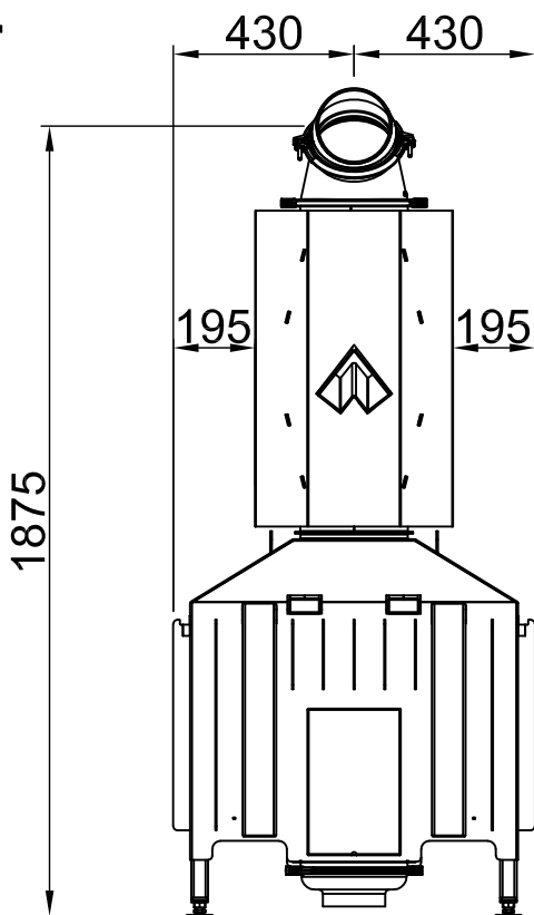
~1:20 Thermobox, schmal
